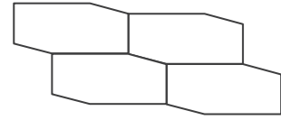
KYTOS 380 | 855 x 380 x 15/16 mm - 285 x 76 x 15/16 mm
